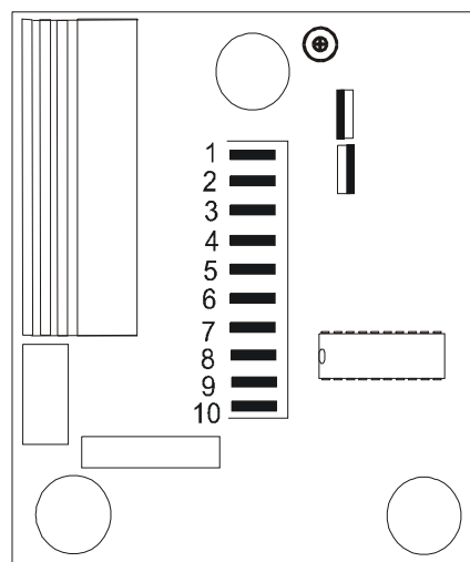
2281 PCB AA3.0
