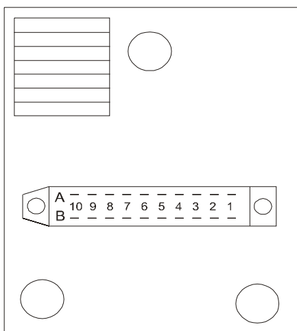
1908 PCB EW22GAN
