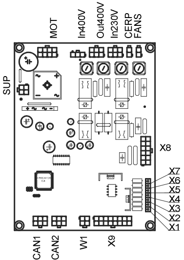
PCB CHOPPER - detail
