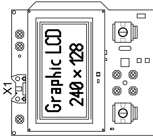
PCB - FRONT PANEL, detail
